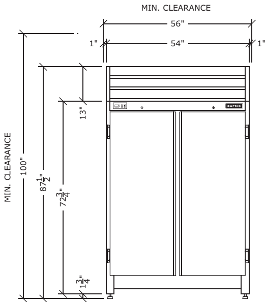
FRONT ELEVATION
