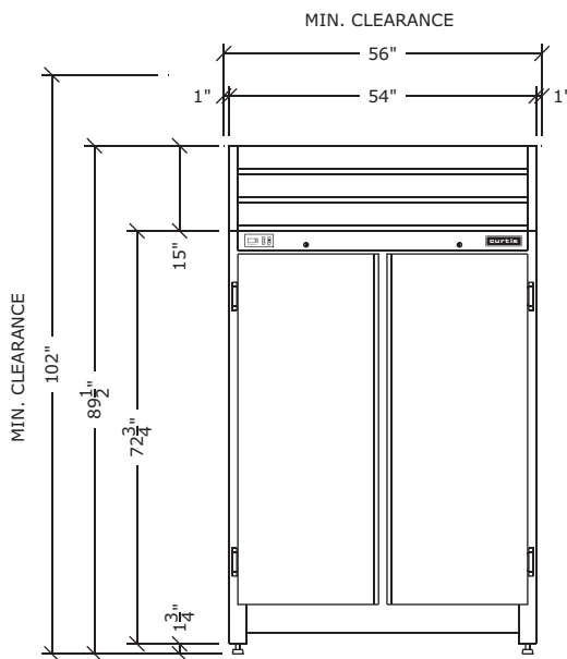
FRONT ELEVATION
