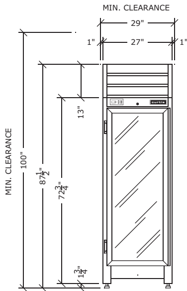
FRONT ELEVATION
