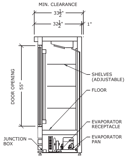
SECTION
